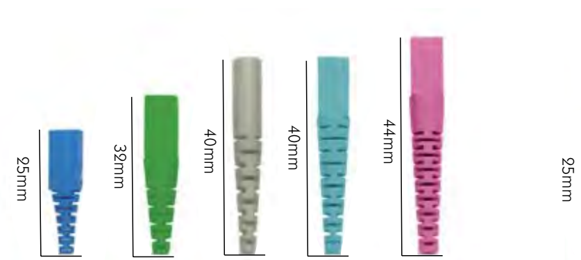
SC 0.9mm Boot
