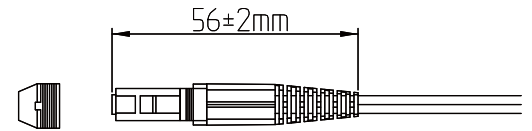
MTRJ Connector
