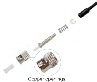
ST 0.9mm Connector
